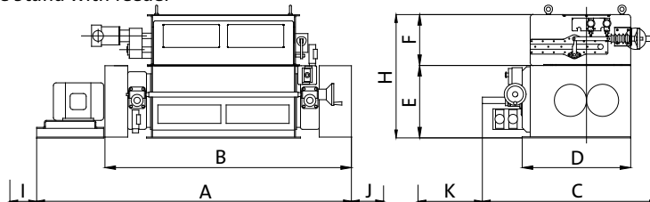
Single Stand with feeder
