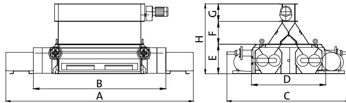
Double Stand with feeder and divider
